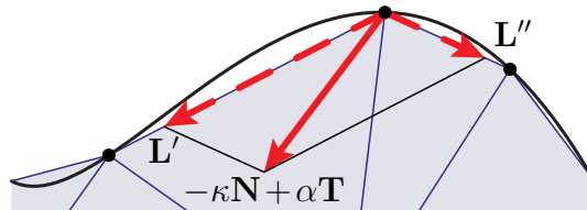
Figure 2.4. The same discrete approximation for a smooth curve as in Figure 2.3. Here, the pulling forces \mathbf{L}' and \mathbf{L}'' are scaled to be proportional to the corresponding side length, according to the rubber-band formulation in equation (2.85). The resulting force contains a tangential component \alpha \mathbf{T} which depends on the length difference of the participating element sides. Its precise magnitude is unspecified.
