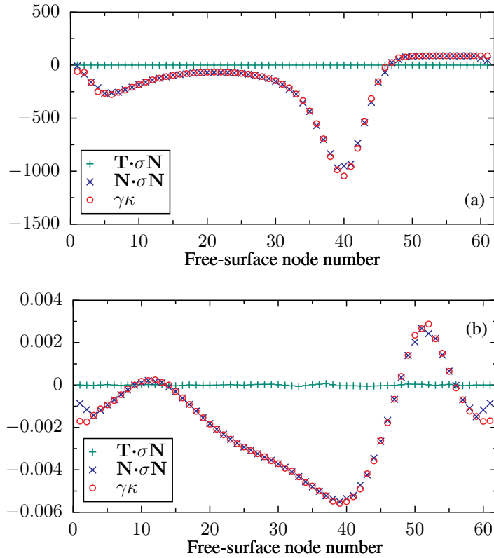
Figure 2.14. The stress balance at the free surface is found to be satisfied. Depicted are the tangential and the normal components of the forces at the surface, together with the reconstruction of the curvature for the droplets in Figure 2.12 (here, panel a) and Figure 2.13 (panel b). The tangential component of the normal stress is found to vanish, while its normal component equals the tension force. For the curvature, the reconstruction technique has been tested in Figure 2.8. The numbering of the free-surface nodes starts with the left contact point and ends with the right one. As in Figure 2.8, in the proximity of the contact nodes the reconstruction technique causes errors.
