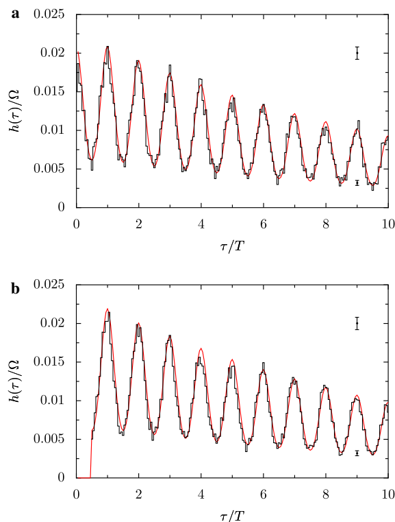
Fig. 3. The histogram (steplike graph) of the interspike intervals resulting from a simulation of the nonlinear leaky integrate-and-fire model (5) is compared with the interspike interval density h(t) given by Eq. (15) (smooth curve) as a function of the interval duration in units of the driving period T = 2\pi/\Omega for the parameter values a = 0.4 , A = 0.01 , D = 0.003 . The two bars on the right side indicate the largest and smallest occurring statistical errors of the histogram for the density values 0.02 and 0.005, respectively. There are no significant deviations between simulations and theory. In the upper panel (a), the refractory time t_f is zero and in the lower panel (b) it coincides with half the period, t_{\text{ref}} = T/2 . Most evidently, a finite deterministic refractory time suppresses the immediate succession of firing events. Upon closer inspection one finds the probability which is removed by the presence of the refractory state from the short intervals transferred to the longer ones. Local maxima of the interspike interval density are found at integer multiples of the signal period.
